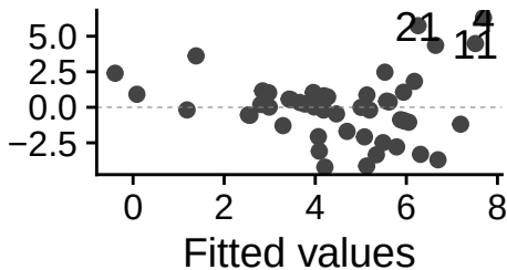
Residuals vs Fitted
